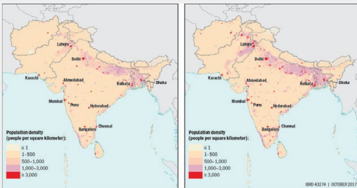
Figure 4.21: Baseline and projected population density in urban areas of South Asia, 2010 and 2050
